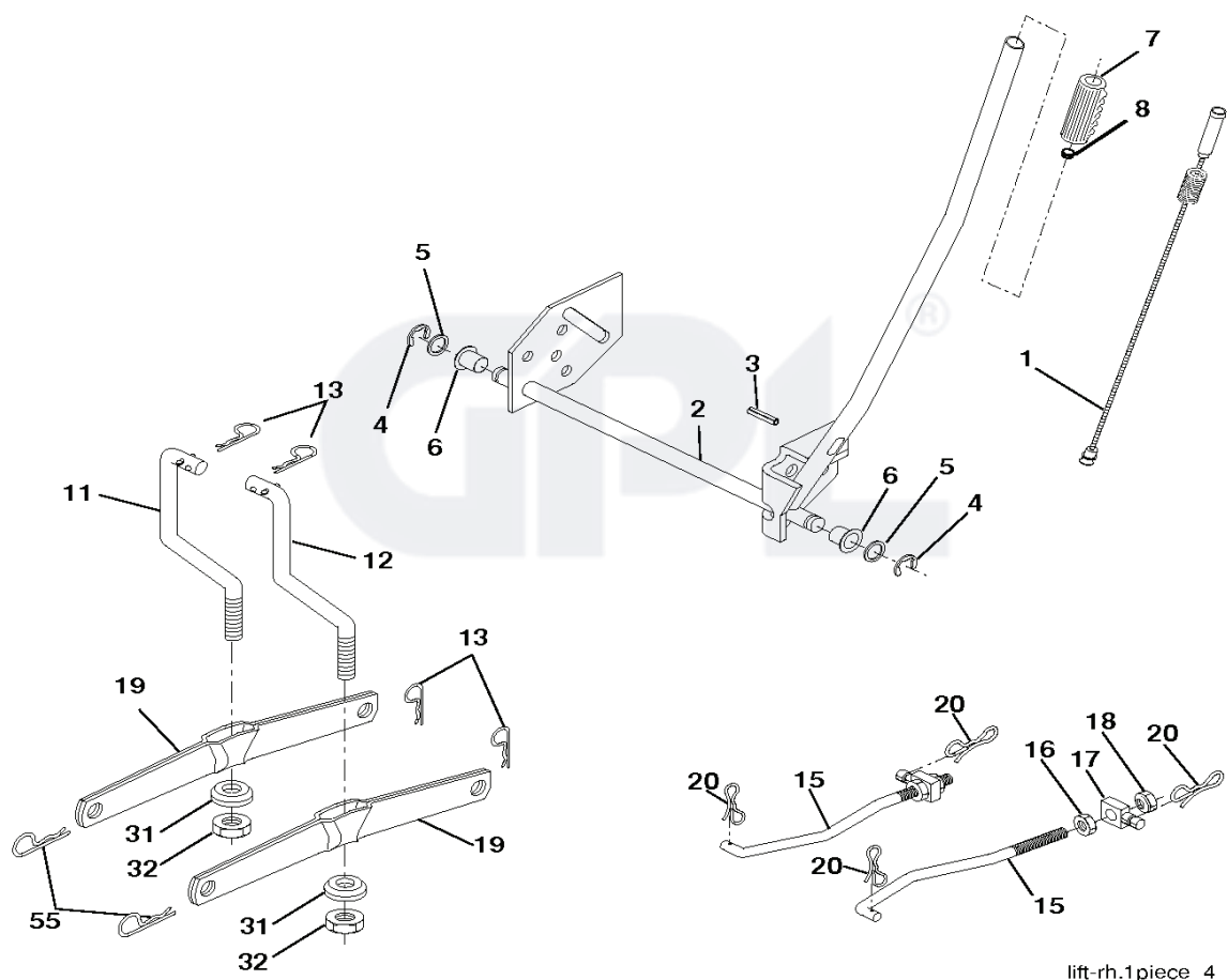
lift-rh.1piece_4
